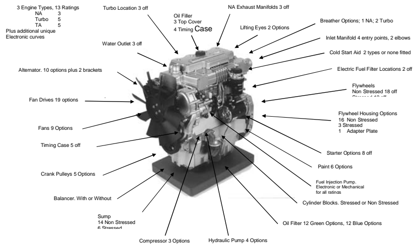
Figure 1 Versions of a diesel engine
